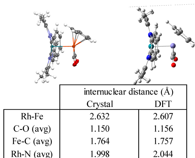
Figure 6. ORTEP representation of (\text{tmtaa})\text{Rh-FeCp}(\text{CO})_2 ( 9 ) structure from single crystal X-ray diffraction with thermal ellipsoids shown on non-hydrogen atoms at 50% probability level, hydrogen atoms shown as open circles, and energy minimization by DFT computations (B3LYP, 3-21G/6-31G*). A table of selected internuclear distances observed in the molecular structure and calculated by DFT is also included.
