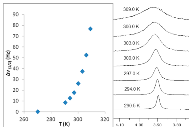
Figure 2. Temperature dependence of the 1 H NMR line width for the cyclopentadienyl ligand in (tmtaa)Rh–CrCp(CO) 3 .
