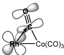
Figure 7. Drawing of the semibridging carbonyl in (tmtaa)Rh-Co(μ-CO)(CO) 3 showing the donation of rhodium dπ into the C≡O π* orbital.
