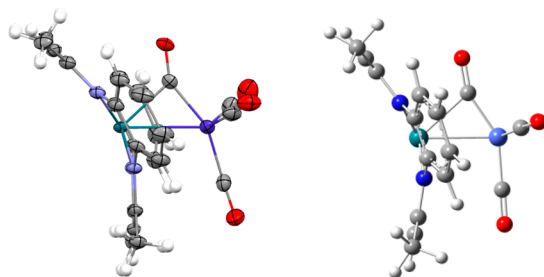
Figure 7. Drawing of the semibridging carbonyl in (tmtaa)Rh-Co(μ-CO)(CO) 3 showing the donation of rhodium dπ into the C≡O π* orbital.
