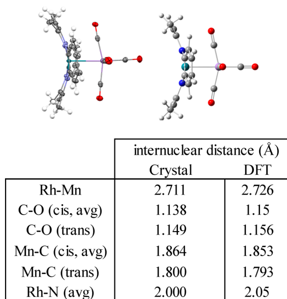
Figure 10. ORTEP representation of the (tmtaa)Rh-Mn(CO) 5 structure from single crystal X-ray diffraction with thermal ellipsoids shown on non-hydrogen atoms at 50% probability level, hydrogen atoms shown as open circles, and energy minimization by DFT computations (B3LYP, 3-21G/6-31G*). A table of selected internuclear distances observed in the molecular structure and calculated by DFT is also included.
