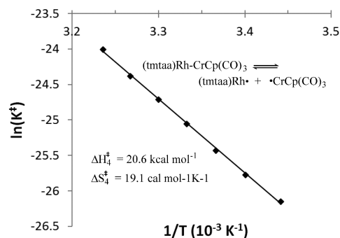
Figure 3. Determination of activation parameters for homolytic dissociation of (tmtaa)Rh–CrCp(CO) 3 into (tmtaa)Rh• and (CO) 3 CpCr• in d 8 -toluene by 1 H NMR line width measurements of the cyclopentadienyl hydrogens ( \Delta H_4^\ddagger = 21 (1) kcal mol -1 , \Delta S_{\text{ex},4}^\ddagger = 19.6 (1.2) cal K -1 mol -1 ).
